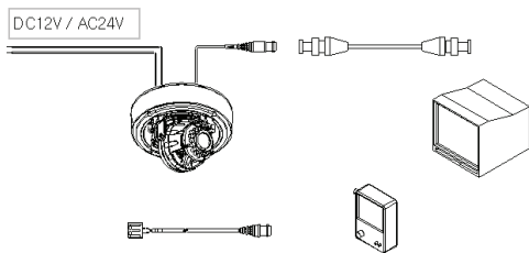
Figure 3.1 Connections with video cable
